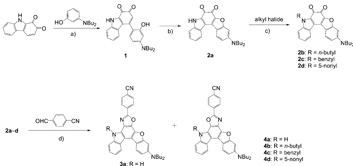
Scheme 1. Synthesis of fluorophores 3 and 4 . a) CuCl 2 , DMSO, 50 °C, 1.5 h, 32%; b) Cu(OCOCH 3 ) 2 , DMSO, 80 °C, 1.0 h, 63%; c) 2b : iodobutane, aq. Na 2 CO 3 , N -methyl-2-pyrrolidinone, 90 °C, 10 h, 23%; 2c : benzyl bromide, aq. KOH, Bu 4 NBr, toluene, reflux, 12 h, 31%; 2d : 5-bromononane, aq. KOH, Bu 4 NBr, toluene, reflux, 10 h, 26%; d) CH 3 COOH, CH 3 COONH 4 , 90 °C, 1–4 h, 55% for 3a , 16% for 4a , 62% for 4b , 63% for 4c , 15% for 4d .
