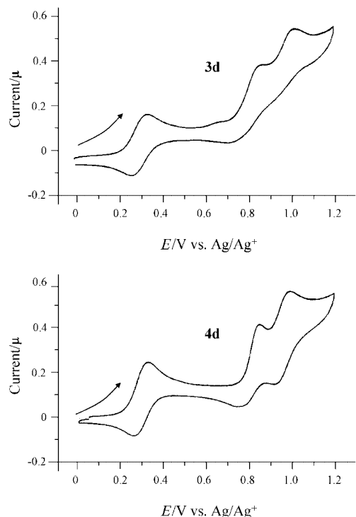
Figure 2. Cyclic voltammograms of compounds 3d and 4d in acetonitrile containing 0.1 M \text{Et}_4\text{NClO}_4 at a scan rate of 20 \text{ mV s}^{-1} .
