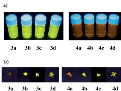
Figure 4. Fluorescence properties of 3a–d and 4a–d , a) in 1,4-dioxane and b) in the solid state.
