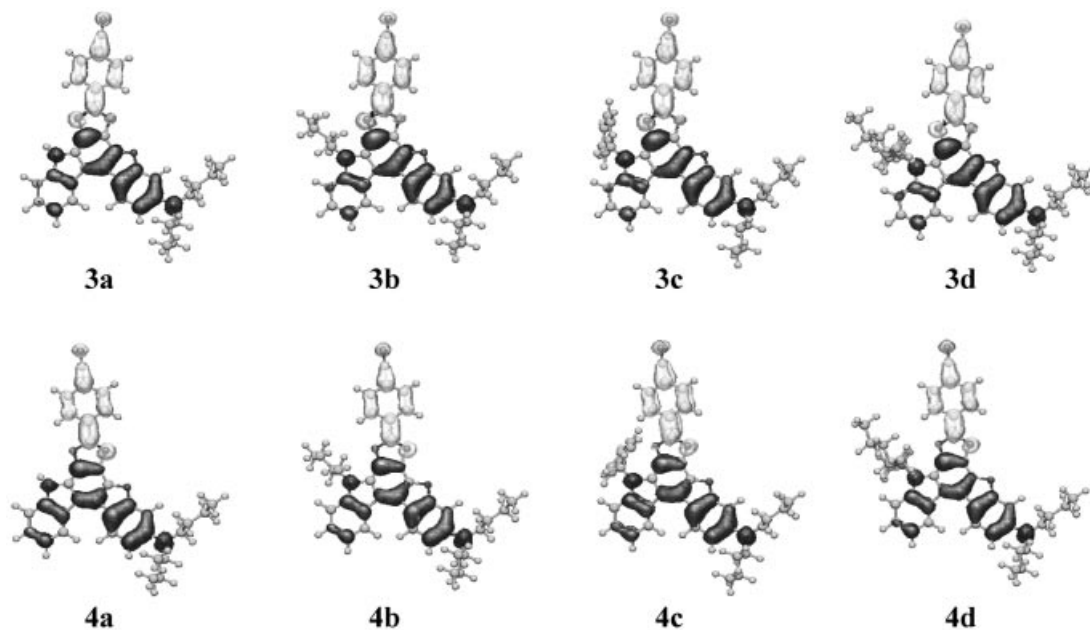
Figure 3. Calculated changes in electron density accompanying the first electronic excitation of 3a–d and 4a–d . The black and white lobes signify decrease and increase in electron density accompanying the electronic transition, respectively. Their areas indicate the magnitude of the electron density change.
