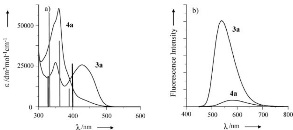
Figure 1. a) Absorption and b) fluorescence spectra of compounds 3a and 4a in 1,4-dioxane. The calculated absorption spectra of 3a and 4a are shown in black and gray lines, respectively.
